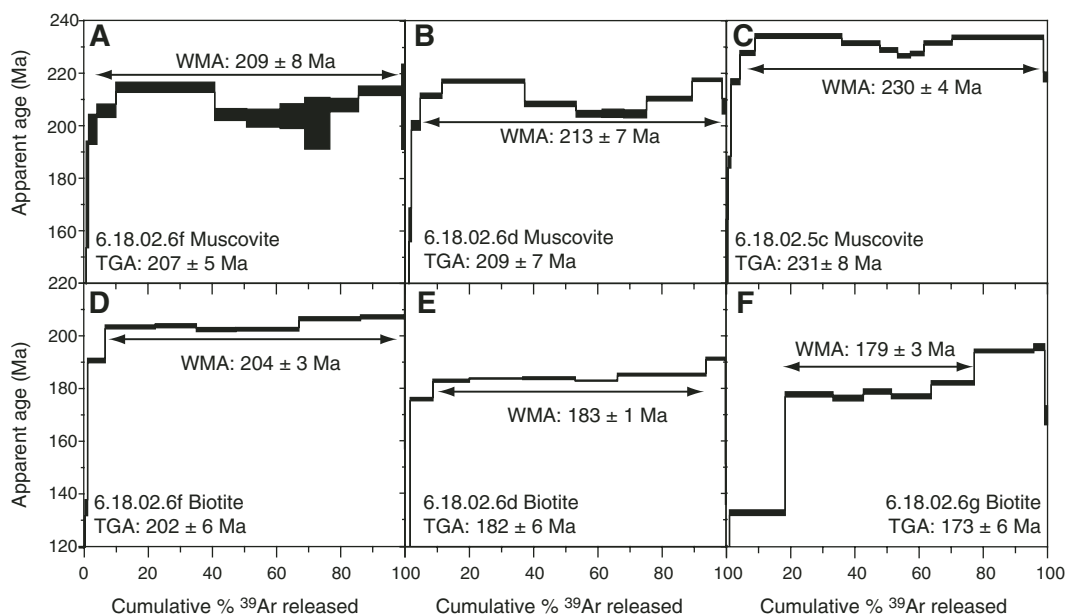
Figure 7. Muscovite and biotite ^{40}\text{Ar}/^{39}\text{Ar} release spectra from Barils hanging wall.
