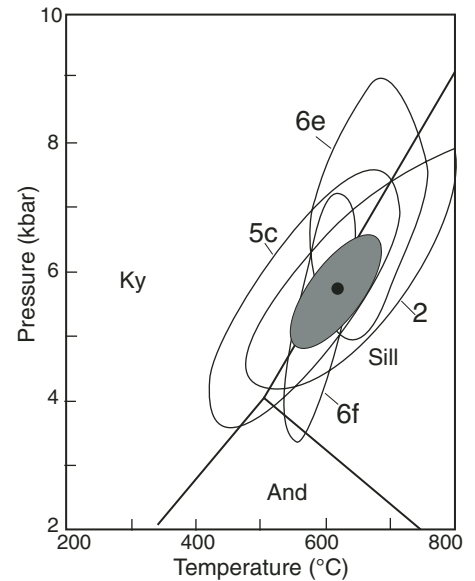
Figure 5. P-T (pressure-temperature) results from Barils hanging wall. Each unfilled error ellipse is the P-T result from a single sample ( 2\sigma ). The average of the four samples for the Barils hanging wall is shown by charcoal-gray filled error ellipse ( 1\sigma ) with a black solid dot in the center at P = 5.75 kbar and T = 615 °C. Sample numbers were abbreviated as follows: 2—6.18.02.2; 5c—6.18.02.5c; 6e—6.18.02.6e; and 6f—6.18.02.6f. Aluminosilicate triple junction shown for reference: Ky—kyanite, Sill—sillimanite, And—andalusite.
