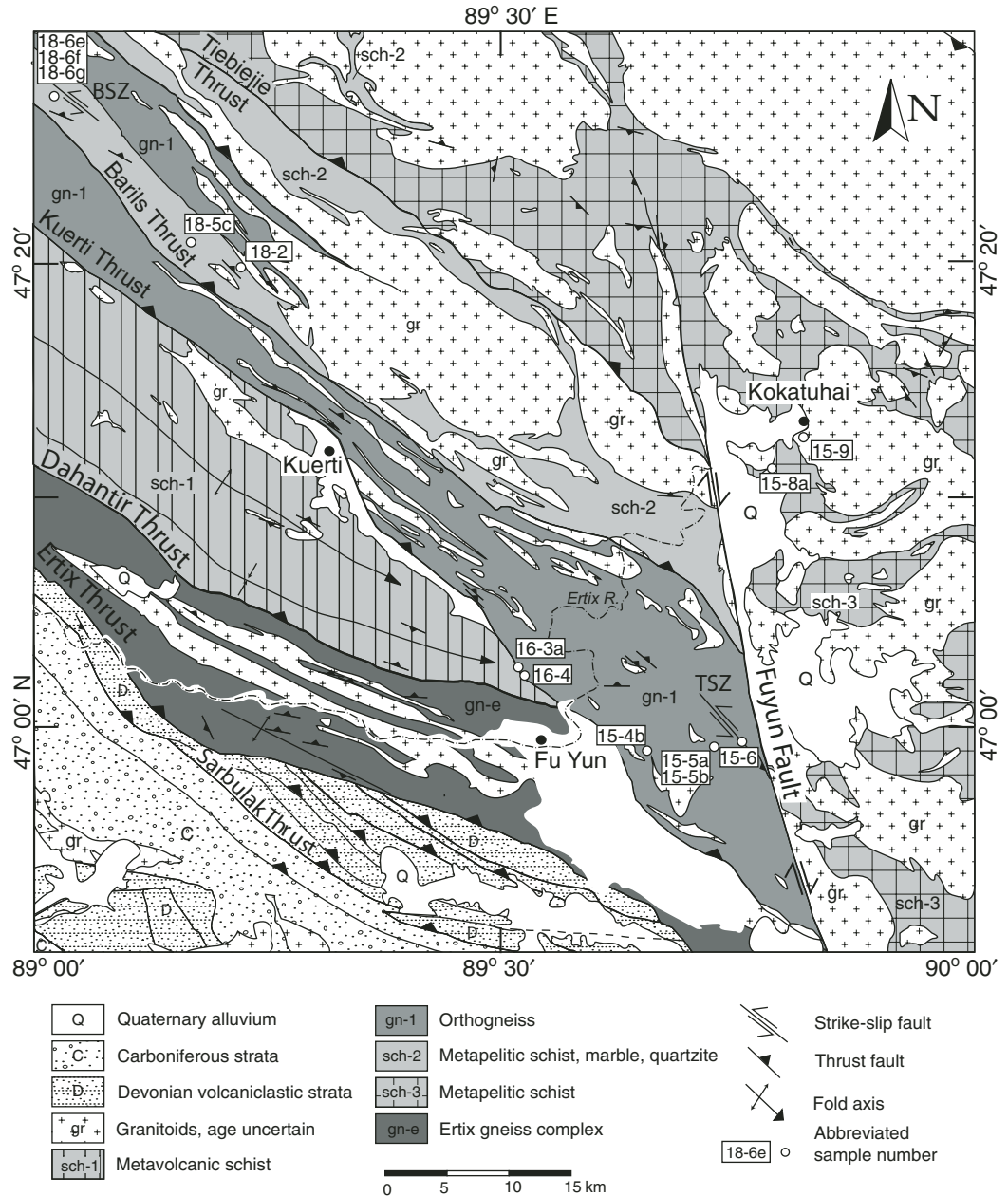
Figure 2. Map of the Fuyun area in the southern Chinese Altai Range, based on a compilation of maps by Xinjiang Bureau of Geology and Mineral Resources (BGMR) (1978, 1993) and our own field observations. Sample sites (small white dots) are accompanied by abbreviated sample labels (e.g., 6.18.02.5c = 18-5c). Labels for strike-slip shear zones are also abbreviated: Balaerqishi Shear Zone—BSZ; Tuhongshat Shear Zone—TSZ.
