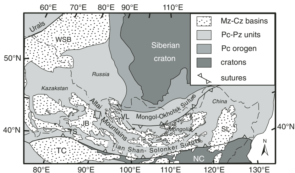
Figure 1. Generalized tectonic map of central Asia. Solid box is location of field area for this study. Abbreviations: TC—Tarim craton; JB—Junggar basin; NC—North China craton; SL—Songliao basin; VL—Valley of the lakes; WSB—West Siberian basin.
