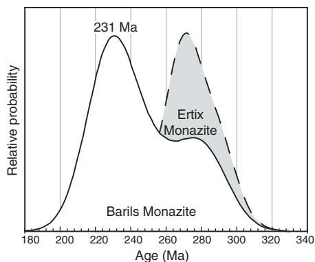
Figure 6. Probability distribution function for monazite from the Barils hanging wall (in white). Gray shaded peak is the probability distribution for monazite ages from the Ertix hanging wall (from Briggs et al., 2007).
