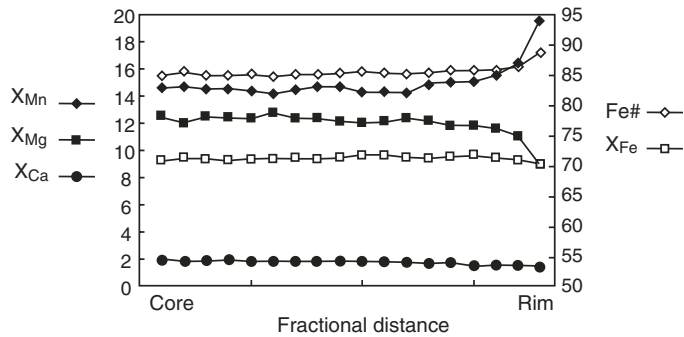
Figure 4. Zoning line from a garnet in a metapelite sample 6.18.02.5c in the Barils hanging wall. Compositional parameters in mole%. X_{Mn} , X_{Mg} , and Fe# show up to 5% variations in the outer 25 \mu\text{m} of the garnet grain. This zoning is compatible with diffusional or retrograde zoning during heating and decompression.
