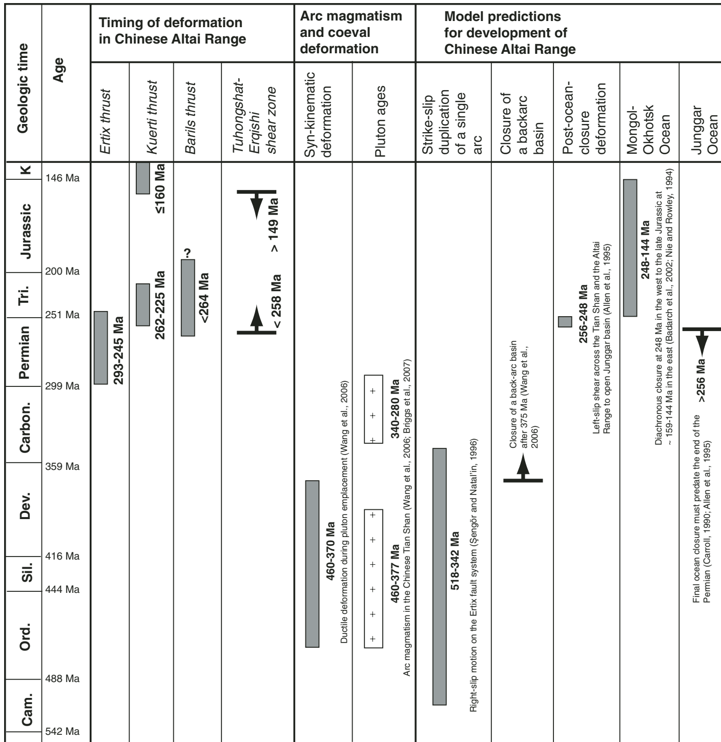
Figure 10. A summary of fault chronology in the context of regional arc magmatism and predictions of tectonic models for the development of the Chinese Altai Range.
