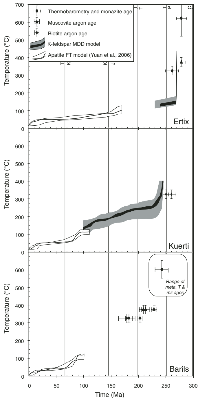
Figure 9. Temperature-time summaries of data from Ertix (top panel), Kuerti (middle panel), and Barils (bottom panel) hanging walls, from this study, Yuan et al. (2004), and Briggs et al. (2007). In the Barils panel, the rounded rectangle shows the full range of ages from individual monazite analyses and retrieved metamorphic temperatures. The average monazite age and metamorphic temperature with standard errors are shown with the ellipse and error bars; the argon ages are paired with assumed closure temperatures (triangles and diamonds). Boundaries between time periods are shown for reference (International Commission on Stratigraphy). Abbreviations: FT—fission track; meta.—metamorphic; MDD—multi-domain diffusion; mz—monazite; T—temperature.
