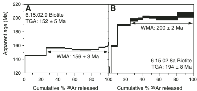
Figure 8. Biotite ^{40}\text{Ar}/^{39}\text{Ar} release spectra for samples from the east side of the Fuyun fault.
