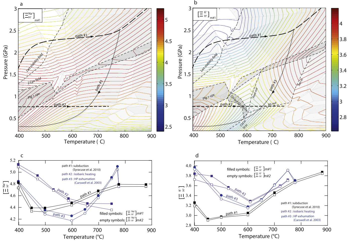
Fig. 5. Contours of activity ratio for selected cations at equilibrium with a devolatilizing metapelite (Fig. 4) for model #1 (pure H 2 O) and model #2 (C-saturated COH fluid, X O = 1/3): a. \mathcal{E}_{\text{H}^+}^{\text{Na}^+} for model #1. It shows the P dependence of \mathcal{E}_{\text{H}^+}^{\text{Na}^+} ratio, reaching a maximum along equilibrium (11). It also shows the T dependence of \mathcal{E}_{\text{H}^+}^{\text{Na}^+} isolines slopes (see text for details). b. \mathcal{E}_{\text{H}^+}^{\text{K}^+} for model #1. The low P domain of biotite–muscovite costability is the prominent feature. In addition, profiles along a subduction (path #1), isobaric heating (path #2), and exhumation (path #3, Carswell et al., 2003) paths for the ratio \mathcal{E}_{\text{H}^+}^{\text{Na}^+} (model #1, filled symbols and model #2, empty symbols) (c) and the ratio \mathcal{E}_{\text{H}^+}^{\text{K}^+} (d) are indicated. Note that some high- T portions of paths #2 and #3 cross the solidus and would require fluid addition (ca. 2 wt%) to maintain equilibrium. This shows the negligible effect of the addition of C on the values and shape of the standard-state variables \mathcal{E}_{\text{H}^+}^{\text{Na}^+} and \mathcal{E}_{\text{H}^+}^{\text{K}^+} .
