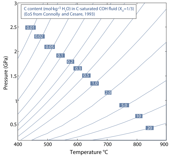
Fig. 2. Contour plot of C molality ( \text{mol}\cdot\text{kg}^{-1} H 2 O) in a C-saturated (graphite) COH fluid at X_0 = 1/3 . The EoS used is from Connolly and Cesare (1993), and it assumes that the solid C phase is perfectly crystalline graphite, refer to Appendix B for details. The C molality spans a large range ( 10^{-3} to >10 molal) and reaches the highest values at elevated T and lower P as can be expected from the weakly polar nature of H 2 O at these conditions, i.e. where ( \epsilon_r ) H 2 O is lowest (Fig. 1). The \log f(\text{O}_2) of this fluid ranges between -2.5 (elevated T and low P ) and 0 log units (elevated P and low T ) below the fayalite–magnetite–quartz (FMQ) equilibrium \log f(\text{O}_2) . Interestingly, the solubility of CaCO 3 in pure H 2 O (Caciagli and Manning, 2003) displays comparatively limited variations around 0.01 to 0.3 molal in this P - T range, and only equals or exceeds that of C at the high P and low T conditions typical of the blueschist–lawsonite facies (cf. Fig. 4) where ( \epsilon_r ) H 2 O is highest (Fig. 1). This geochemical feature is noteworthy given the dramatically different structure, properties and kinetics of dissolution of these important C-bearing minerals.
