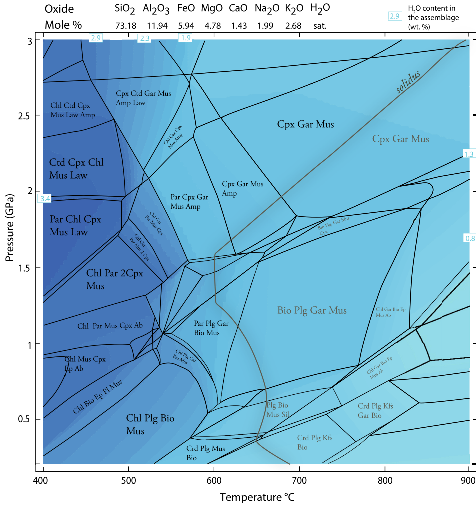
Fig. 4. P – T section in the NCKFMASH system for a model pelite indicating the location of the main mineral assemblages. Blue shading in the background indicates the isopleth of the \text{H}_2\text{O} content present in the rock at equilibrium (wt%). For example, the 400–600 °C and 1–3 GPa interval correspond to the blueschist–eclogite transition, characterized by significant \text{H}_2\text{O} loss by the mineral assemblage (>3.4 wt% at blueschist conditions to ca. 1.5 wt% \text{H}_2\text{O} at eclogite conditions) in response to continuous devolatilization of hydrous-phases, i.e. lawsonite, chloritoid, chlorite and glaucophane. Black contours delineate distinct mineralogical phase fields and sub-solidus assemblages are indicated in black. Super-solidus assemblages, metastable with respect to a melt phase, are indicated in dark green. The position of the wet-solidus is also indicated. Starting composition is indicated above the figure (adapted from Caddick and Thompson, 2008) and solution models used can be found in Appendix C.
