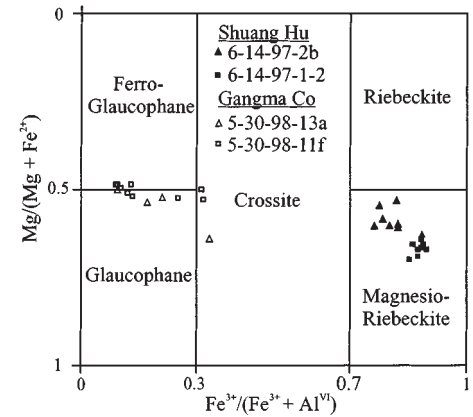
Figure 4. Compositions of sodic amphibole in four samples of epidote blueschists from Shuang Hu and Gangma Co areas. Points plotted are single electron-microprobe spot analyses.
