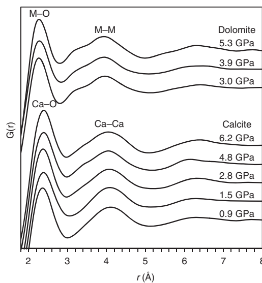
Figure 4 | Structure of calcite and dolomite melts at high pressures.
