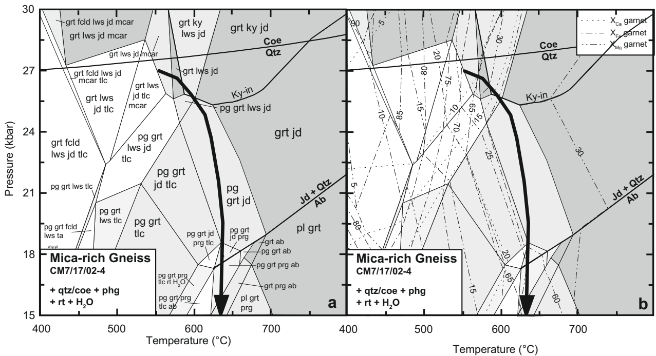
Fig. 9. (a) P-T pseudosection phase diagram summarizing the phase relations in the mica-rich gneiss (CM7/17/02-4). Thin solid lines separate different mineral assemblages. Quartz or coesite, phengite and rutile are predicted in all assemblages. The thick dark lines denote important reaction boundaries: jadeite + quartz = albite, coesite = quartz and first appearance of kyanite. The thickest black line is the P-T path calculated for the mafic eclogite (Fig. 4). Mineral abbreviations according to Kretz (1983) except coe = coesite and phg = phengite. (b) The same pseudosection with mineral assemblages removed for clarity. Dashed lines are calculated isopleths for Ca, Mg and Fe mole fractions in garnet.
