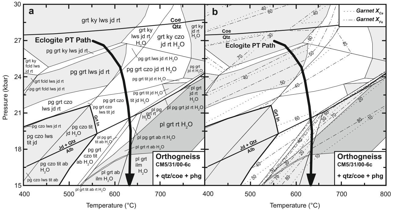
Fig. 8. (a) P-T pseudosection phase diagram summarizing the phase relations in the orthogneiss (CM5/31/00-6c). Thin solid lines separate mineral assemblages. Quartz or coesite and phengite are predicted in all assemblages. The thick dark lines denote important reaction boundaries: jadeite + quartz = albite, coesite = quartz and the first appearance of garnet. The thickest black line is the P-T path calculated for the mafic eclogite (Fig. 4). Mineral abbreviations according to Kretz (1983) except coe = coesite, phg = phengite and tit = titanite. (b) The same pseudosection with mineral assemblages removed for clarity. Dashed lines are calculated isopleths for Ca and Fe mole fractions in garnet.
