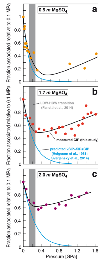
Figure 2 Fraction of \text{MgSO}_4 associated at 21 \pm 1^\circ\text{C} relative to that at ambient pressure, as determined by Raman spectroscopy and thermodynamic modelling, for 0.5 (a), 1.7 (b), and 2 molal solutions (c). Thick black lines are trend lines for the fraction of CIP from Raman spectroscopic data fit by eye. Blue lines denote the fraction of the sum of the CIP, RAN and 2SIP ion pairs calculated from a thermodynamic model based on the DEW model (Sverjensky et al. , 2014) and the Helgeson-Kirkham-Flowers ion activity model (Helgeson et al. , 1981). The comparison assumes that the proportionality between equilibrium constants associated with expelling the \text{H}_2\text{O} molecules between ions is constant and independent of pressure. This assumption yields a minimum difference in predicted and observed CIP. The shadowed band is the pressure range of the LDW-HDW transition at about 20^\circ\text{C} (Fanetti et al. , 2014).
