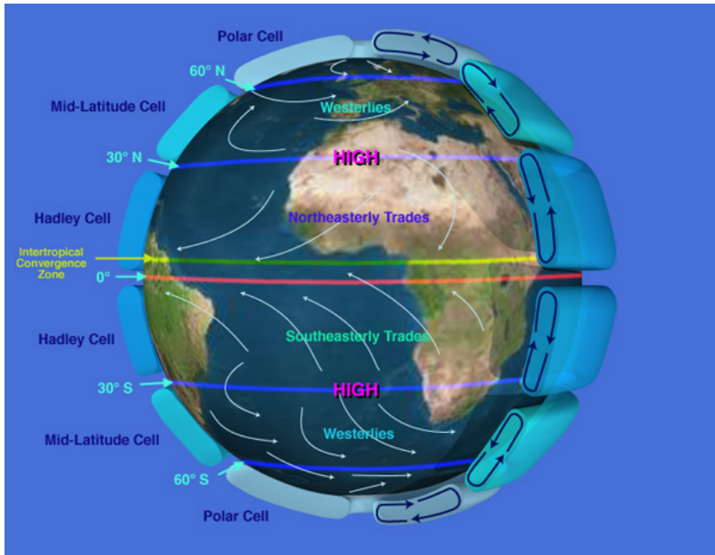
Figure from NASA, Public Domain, http://sealevel.jpl.nasa.gov/overview/climate-climatic.html
