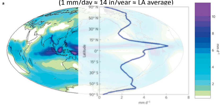
GPCP global precipitation database, Huffman et al. 2009; http://onlinelibrary.wiley.com/doi/10.1029/2009GL040000/full . Graphic from Frierson et al. 2013; https://www.nature.com/articles/ngeo1987/figures/1
