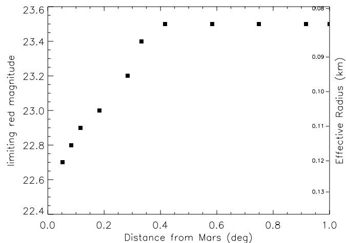
FIG. 4.—The 50% efficiency detection red limiting magnitude of the survey vs. distance from Mars. Scattered light is only significant starting at about 15' from Mars. The calculation of the effective radius assumes an albedo of 0.07.
