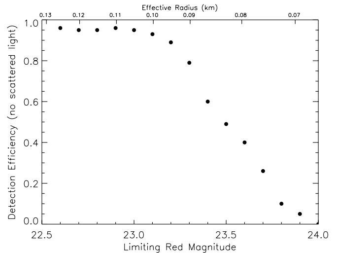
FIG. 2.—Detection efficiency of the moving-object search computer program vs. the apparent red magnitude. The 50% differential detection efficiency is at about 23.5 mag. The differential efficiency was determined by how many artificially generated moving objects with motions similar to that of Mars were found by the program at a given magnitude. Magnitude bins were separated by 0.1. This efficiency is for no significant scattered light in the fields. The calculation of the effective radius assumes an albedo of 0.07.
