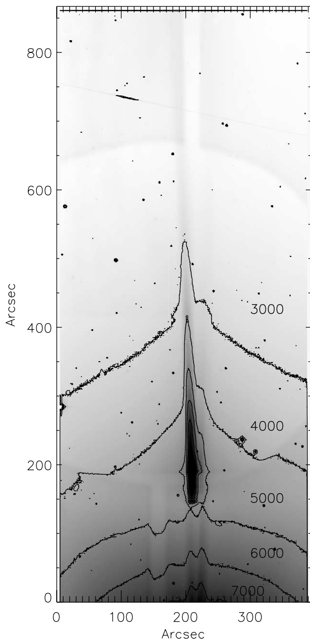
FIG. 3.—Contour plot of a survey image close to Mars to show the scattered light. The contours show 7000:6000:5000:4000:3000 surface brightness contours, where the nominal background sky level away from the planet was near 2000 counts. Mars is about 3' south from the bottom of the plotted region. The vertical spike is caused by diffraction from the telescope's support structure. The image color map has been inverted so that higher counts are darker. The color map was also scaled logarithmically to bring out more detail between the top and bottom of the image.
