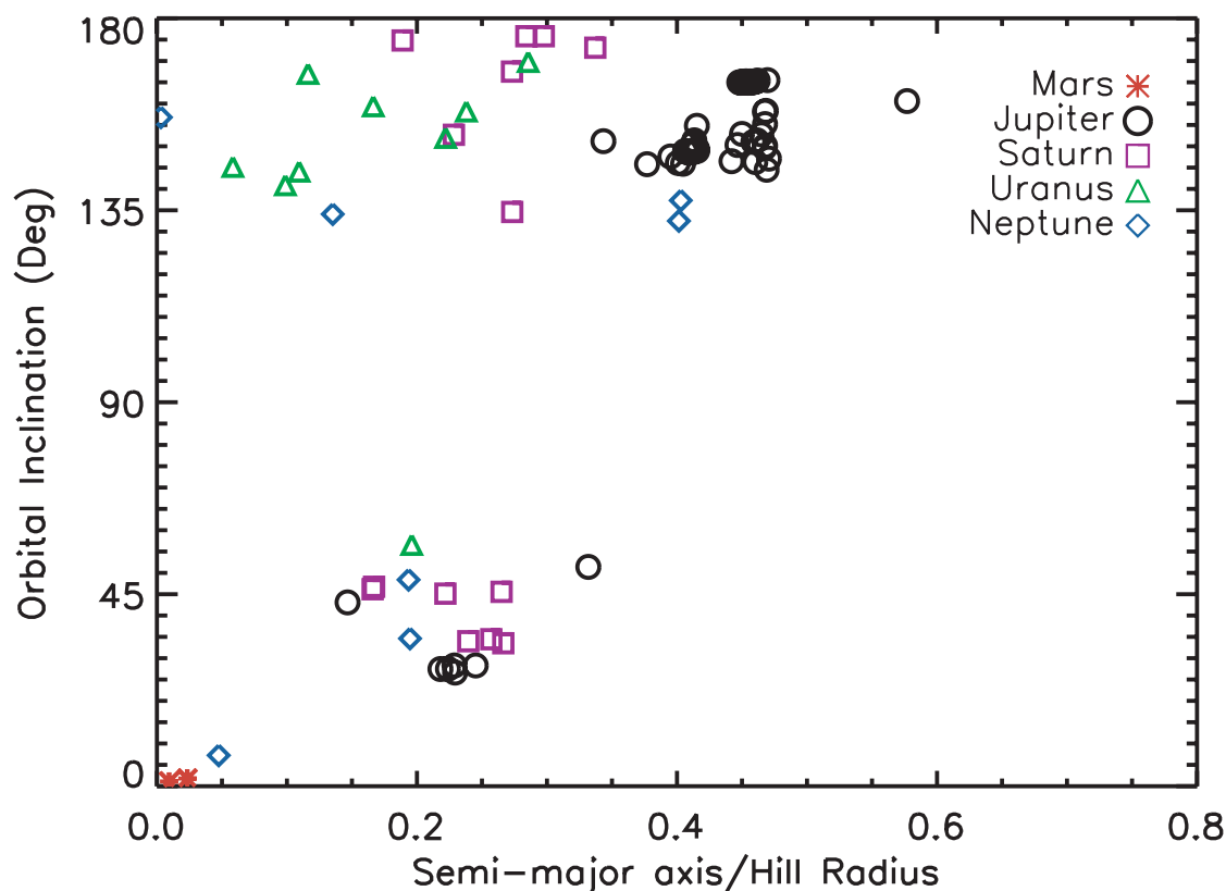
FIG. 5.—Comparison of the known irregular satellites of the giant planets with Mars's two known satellites. The horizontal axis is the ratio of the satellite's semimajor axis to the respective planet's Hill radius. The vertical axis is the inclination of the satellite to the equator of its planet. Only Nereid, of Neptune, is close to the position of the known Martian satellites in this parameter space.
