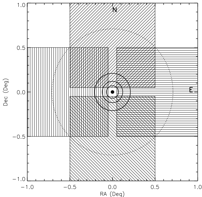
FIG. 1.—Area searched around Mars for satellites using the Canada-France-Hawaii Telescope. Four fields were imaged three times each on two separate nights (UT 2003 July 5 and 7) for a total of 24 images. The black dot at the center represents Mars's position. The dot is larger than the apparent diameter of Mars and incorporates the orbits of Phobos and Deimos. The four different hatched squares represent the four fields imaged around Mars on both nights. Overlapping hatches show where some of the fields overlapped in coverage. The dotted circle shows the Hill sphere of Mars to our line of sight. The scattered light from Mars was not a problem for most of the images but became quickly dominant very near Mars. The inner solid circles show where scattered light became significant compared with the normal sky background. At the outer solid circle, near 0^{\circ}20' , the background was about 1.5 times higher, while at the middle solid circle the background was about 2 times higher and at the inner solid circle the background was about 3.75 times higher than the nominal sky background.
