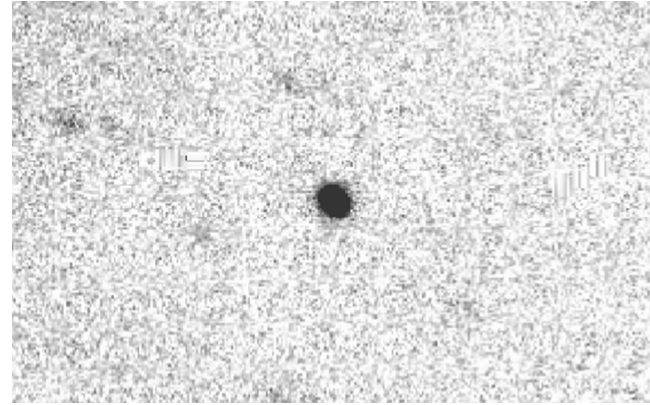
Figure 8.8. 2003 EH 1 in a 360 s R-band image taken at Keck on UT 2013 October 2. No coma or tail is visible on the object having an FWHM of 0''.86 in the frame of 40'' \times 25'' . R = 2.1 AU, \Delta = 2.0 AU and \alpha = 27.6^\circ . From Kasuga and Jewitt (2015).
