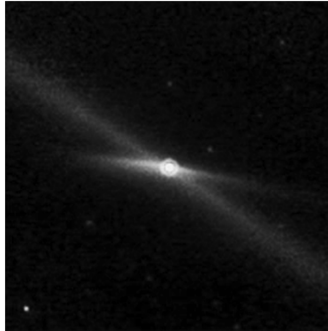
Figure 8.10. The 24\ \mu\text{m} infrared image of comet 2P/Encke obtained in 2004 June by the Spitzer Space Telescope. The image field of view is about 6' and centered on the nucleus. The near horizontal emission is produced by recent cometary activity, and the diagonal emission across the image is the meteoroid stream along the orbit (Kelley et al., 2006; see also Reach et al., 2007). Courtesy NASA/JPL-Caltech/M. Kelley (Univ. of Minnesota). (A black and white version of this figure will appear in some formats. For the colour version, please refer to the plate section.)
