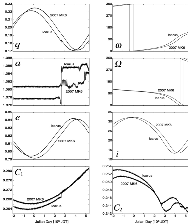
Figure 8.11. Dynamical evolution process of 1566 Icarus and 2007 MK 6 in JTD. The orbital elements ( q , a , e , \omega , \Omega and i ) and the C_1 and C_2 integrals are plotted (cf. Table 8.1). Time-shifting is only \sim 1,000 yr. From Ohtsuka et al. (2007).
