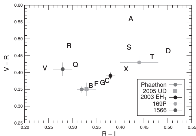
Figure 8.14. The same as Figure 8.13 but in the R - I vs. V - R color plane. The color of the Sun is exactly coincident with that of 2005 UD. (A black and white version of this figure will appear in some formats. For the colour version, please refer to the plate section.)
