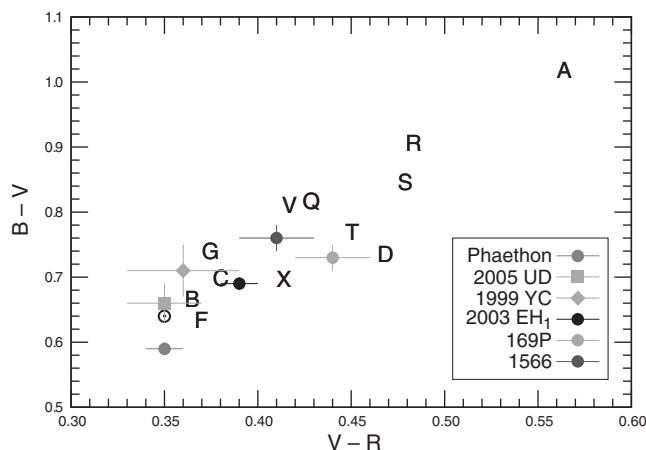
Figure 8.13. Color plots of V - R vs. B - V showing parent bodies (filled symbols) from Table 8.2, and Tholen taxonomic classifications (Tholen, 1984), as tabulated by Dandy et al. (2003). The color of the Sun (red circle) is also plotted. (A black and white version of this figure will appear in some formats. For the colour version, please refer to the plate section.)
