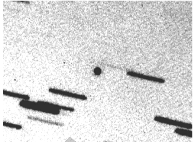
Figure 8.9. Comet 169P/NEAT in a 600 sec, r'-band image taken at the Dominion Astrophysical Observatory 1.8 m telescope on UT 2010 February 17. The frame size is 200'' \times 150'' . No coma or tail is visible on the object having an FWHM of 2.8'' . R = 1.43 AU, \Delta = 0.47 AU and \alpha = 16.1^\circ . From Kasuga et al. (2010).
