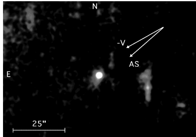
Figure 8.12. 2003 WY 25 (=289P/Blanpain) imaged in R-band, 500 sec integration at R = 1.6 AU, \Delta = 0.7 AU and \alpha = 20.7^\circ using UH2.2 on UT 2004 March 20. A faint coma is apparent, extending to the southeast. Arrows show the directions of the negative heliocentric velocity vector (marked “-V”) and the anti-solar direction (“AS”). The estimated radius \sim 160 m is the smallest active cometary parent ever observed. From Jewitt (2006). (A black and white version of this figure will appear in some formats. For the colour version, please refer to the plate section.)
