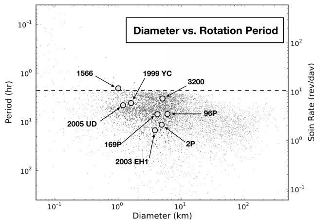
Figure 8.15. Diameter versus rotational period for asteroids (dots) and the parent bodies of meteoroid streams (large circles). The asteroid data are taken from Chang et al. (2015) while the parent body parameters are listed in Table 8.2. The horizontal dotted line shows the spin barrier period of \sim 2.2 hr (e.g. Warner et al., 2009) and asteroid 1566 Icarus rotates nearby.
