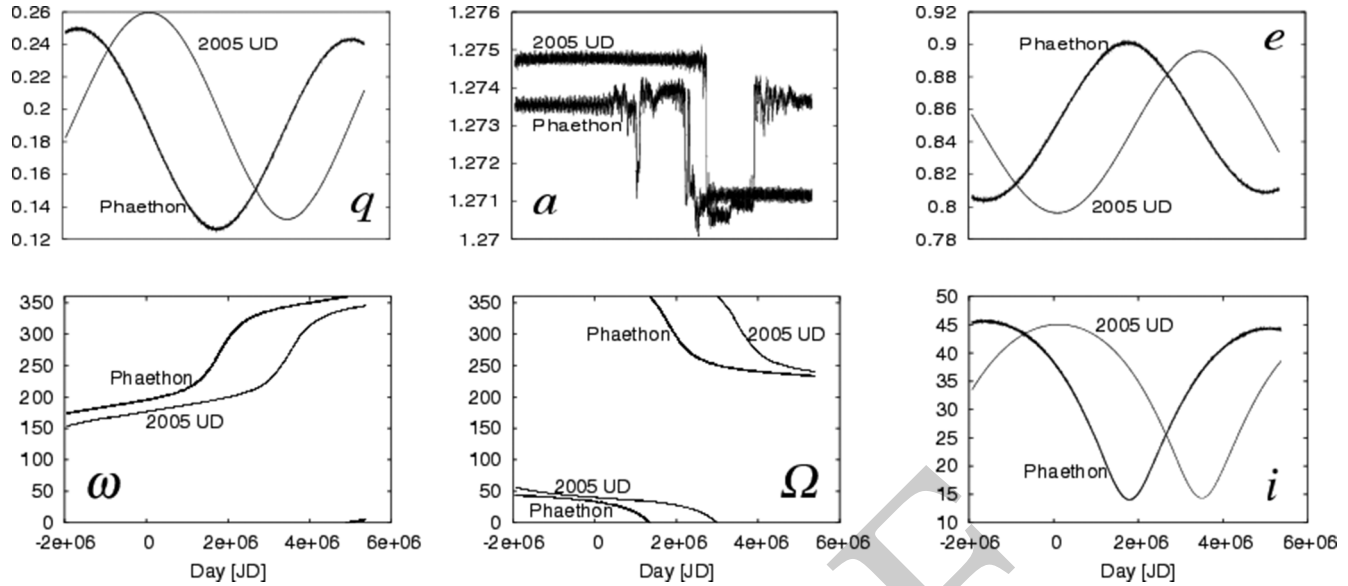
Figure 8.4. Dynamical evolution of (3200) Phaethon and 2005 UD for the six orbital elements, representing similar behavior with a time-shift of \sim 4600 yr. The abscissa shows time in Julian Terrestrial Date (JTD). From Ohtsuka et al. (2006), reproduced with permission © ESO.
