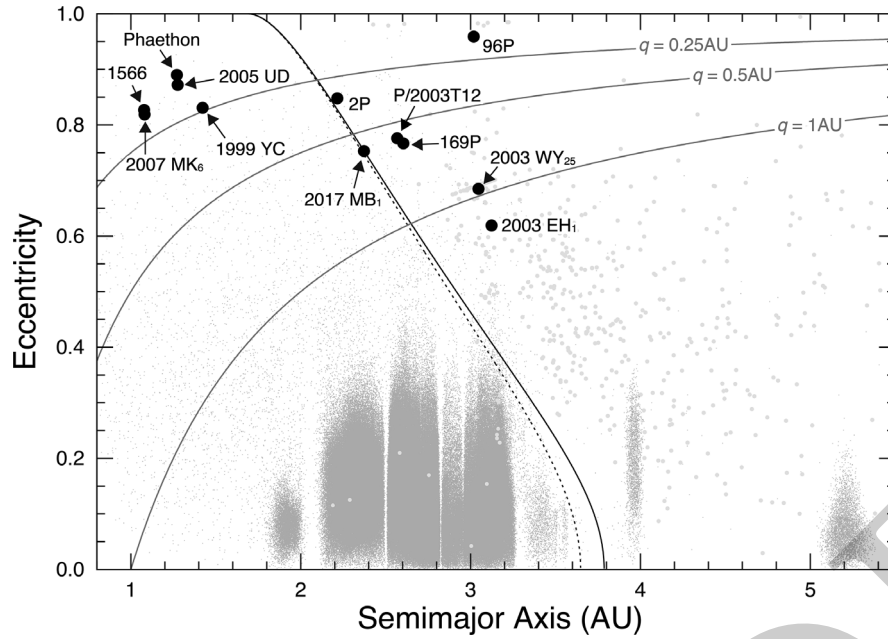
Figure 8.1. Distribution of the parent bodies (large numbered dots) in the semimajor axis versus orbital eccentricity plane (cf. Table 8.1). The distributions of asteroids (fine gray dots) and comets (larger gray dots) are shown for reference. The lines for T_J = 3.08 with i = 0^\circ (solid black curve) and with i = 9^\circ (dotted black curve) broadly separate asteroids and comets. Perihelion distances q = 0.25, 0.5 and 1 AU are shown as solid gray curves. (A black and white version of this figure will appear in some formats. For the colour version, please refer to the plate section.)
