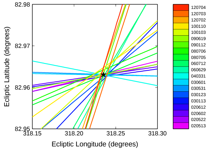
Figure 3. Constraints on spin axis orientation from 20 epochs of correlation maxima observed at low zenith angles (subset identified with an asterisk in Table 1). Epochs are color-coded according to the scale bar at right. The orientation of each line is dictated by the ecliptic longitude of the projected baseline at the corresponding epoch. The individual constraints appear as lines on the celestial sphere because a rotation of the spin vector of Mercury about an axis parallel to the projected baseline does not result in a substantial change in the epoch of correlation maximum. Observations at a range of baseline geometries determine the spin axis orientation in two dimensions. The best-fit spin-axis orientation is marked with a star.
