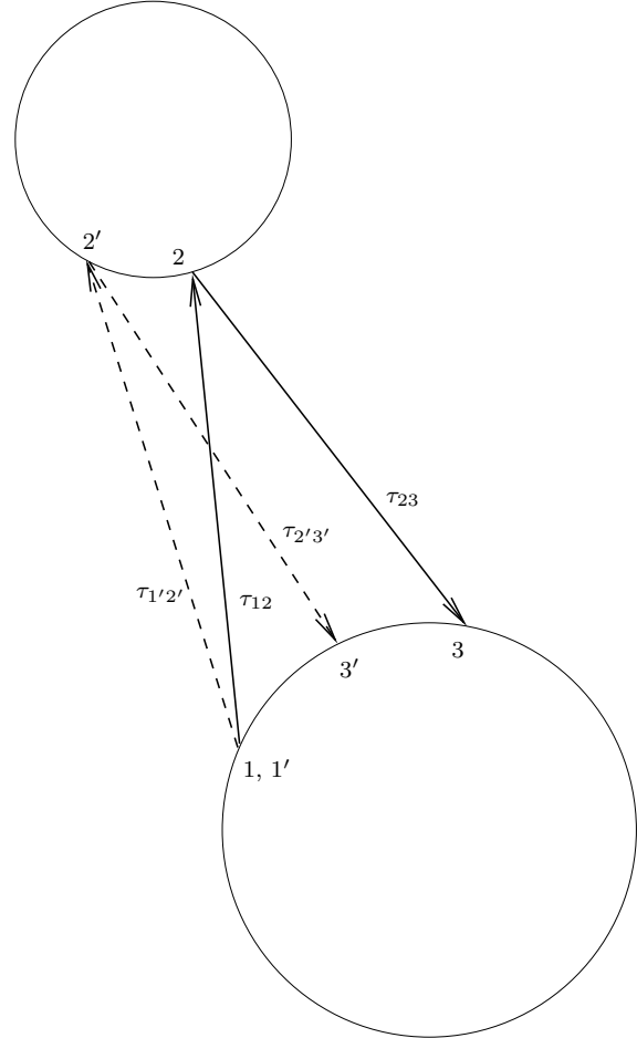
Figure 10. The geometry of the speckle displacement problem involves one transmit station (1 and 1'), two receive stations (3 and 3'), six epochs of participation (two transmit epochs, two bounce epochs, two receive epochs), and four light-time quantities ( \tau_{ij} ). For simplicity, the substantial spin and orbital motions of the planets that occur between the first transmit epoch and the last receive epoch are not shown.
