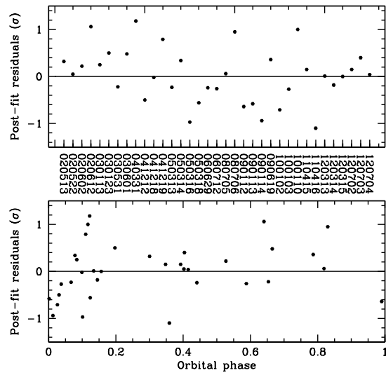
Figure 6. Post-fit residuals from the one-parameter libration fit shown as a function of observing date (top) and orbital phase (bottom), where 0 and 1 mark pericenter. Each residual is the observed minus computed quantity, divided by the corresponding measurement uncertainty.
