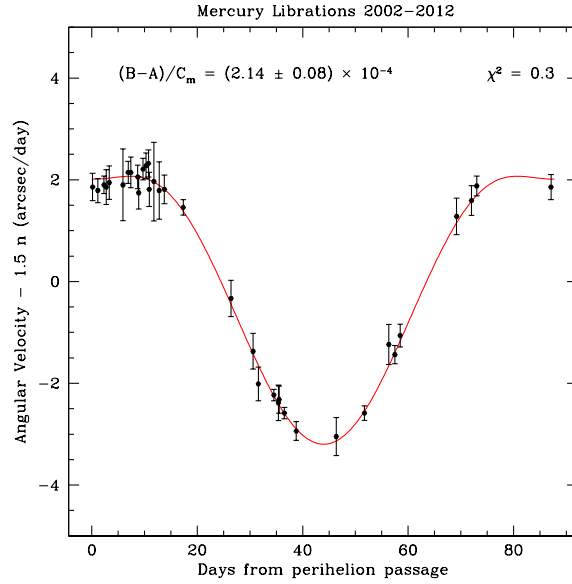
Figure 5. Mercury librations revealed by 35 instantaneous spin rate measurements obtained between 2002 and 2012. The measurements with their one-standard-deviation errors are shown in black. A numerical integration of the torque equation is shown in red. The flat top on the angular velocity curve near pericenter is due to the momentary retrograde motion of the Sun in the body-fixed frame and corresponding changes in the torque. The amplitude of the libration curve is determined by a one-parameter least-squares fit to the observations, which yields a value of (B - A)/C_m = (2.14 \pm 0.08) \times 10^{-4} with reduced \chi^2 of 0.3.
