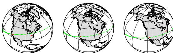
Figure 1. Radar echoes from Mercury sweep over the surface of the Earth during the 2002 May 23 observations. Diagrams show the trajectory of the speckles one hour before (left), during (center), and one hour after (right) the epoch of maximum correlation. Echoes from two receive stations (red triangles) exhibit a strong correlation when the antennas are suitably aligned with the trajectory of the speckles (green dots shown with a 1 s time interval).
