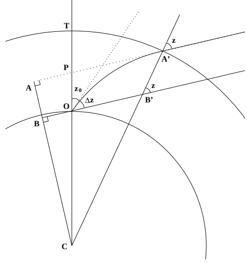
Figure 11. Geometry for atmospheric refraction calculations (see text).
