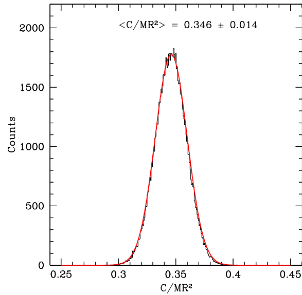
Figure 7. Distribution of C/MR^2 values from 100,000 Monte Carlo trials that capture uncertainties in obliquity, libration amplitude, and gravitational harmonics. C is the moment of inertia of Mercury.
