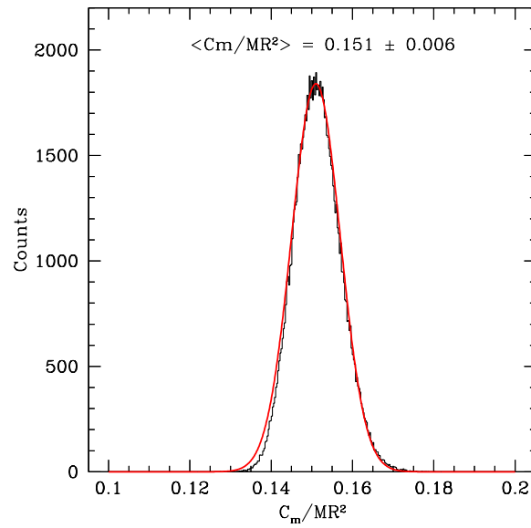
Figure 9. Distribution of C_m/MR^2 values from 100,000 Monte Carlo trials that capture uncertainties in obliquity, libration amplitude, and gravitational harmonics. C_m is the moment of inertia of the outer librating shell. The moment of inertia of the core is C_c = C - C_m .
