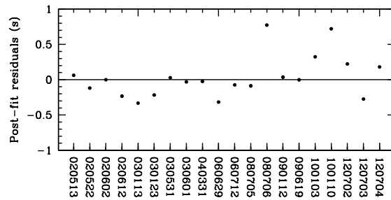
Figure 2. Post-fit residuals, in seconds, from the adopted spin axis orientation fit (20 OC epochs).
