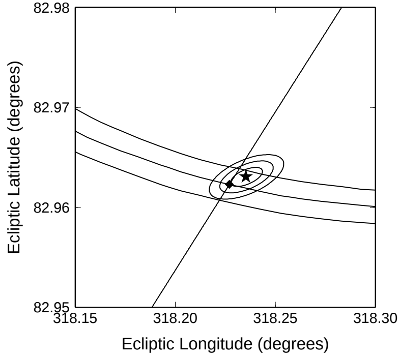
Figure 4. Orientation of the spin axis of Mercury obtained by a least-squares fit to a subset of epochs that are minimally affected by atmospheric refraction. Contours representing 1-, 2-, and 3- \sigma uncertainty regions surrounding the best-fit solution (star) are shown. The contours are elongated along the general direction of the constraints shown in Figure 3. The best-fit obliquity is (2.04 \pm 0.08) arcminutes. The diamond and curved lines show the solution and obliquity uncertainties of Margot et al. [2007]. The oblique line shows the predicted location of Cassini state 1 based on the analysis of Yseboodt and Margot [2006].
