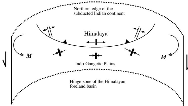
Fig. 18 (continued). Selected models for the development of the Himalayan orogen.
