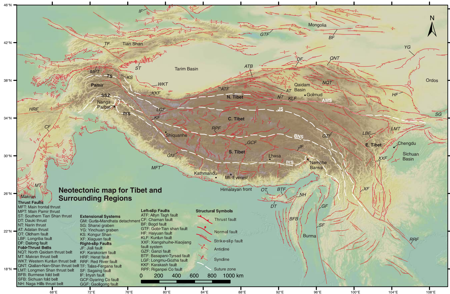
Figure 1. A color-shaded relief map with active to recently active faults related to the Indo-Asian collision zone and surrounding regions. The main sources of information are listed here (i.e., Armijo et al., 1986, 1989; Arrowsmith and Strecker, 1999; Avouac and Peltzer, 1993; Avouac et al., 1993; Burchfiel et al., 1991, 1995, 1999; Cowgill et al., 2000, 2004b; Darby and Ritts, 2002; Darby et al., 2005; Jackson, 1992; Jackson et al., 1995; Jackson and McKenzie, 1984; Kapp and Gynn, 2004; Kirby et al., 2000; Lave and Avouac, 2000; Meriaux et al., 2004, 2005; Murphy et al., 2000; Peltzer et al., 1989; Robinson et al., 2004; Tapponnier and Molnar, 1979; Tapponnier et al., 1981b, 2001; Taylor and Peltzer, 2006; Taylor et al., 2003; ten Brink and Taylor, 2002; Thatcher, 2007; Thompson et al., 2002; Wang and Burchfiel, 2000; Wang et al., 1998; Xu et al., 2008; Yeats and Lillie, 1991; Yin et al., 2008a; Yin and Harrison, 2000), and are augmented by our own kinematic interpretations. Thrust faults have barbs on the upper plate, normal faults have bar and ball on the hanging wall, arrows indicate direction of horizontal motion for strike-slip faults. Dashed white lines are Mesozoic suture zones: IYS—Indus Yalu suture zone; BNS—Bangong Nuijiang suture zone; JS—Jinsha suture zone; SSZ—Shyok suture zone; TS—Tanymas suture zone; AMS—Anyimaqen-Kunlun-Muztagh suture zone.
